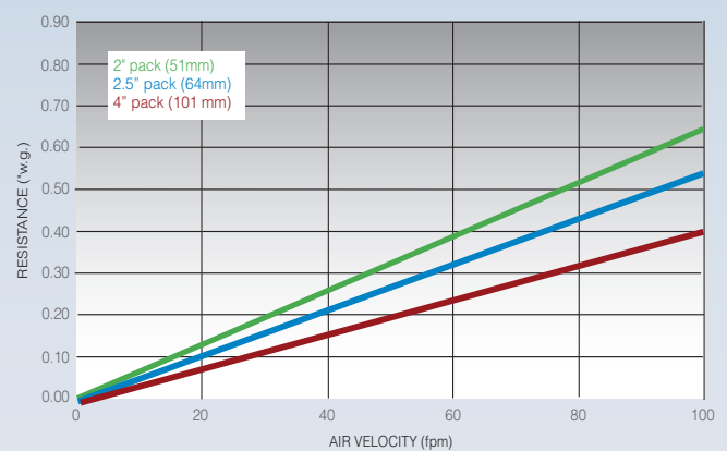
INITIAL RESISTANCE VS. FACE VELOCITY (ULPA)
