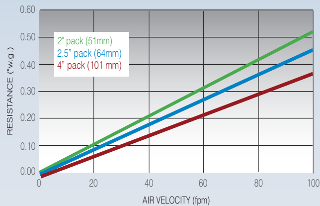
INITIAL RESISTANCE VS. FACE VELOCITY (HEPA)
